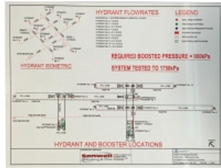
Block Plan 600 x 400mm
